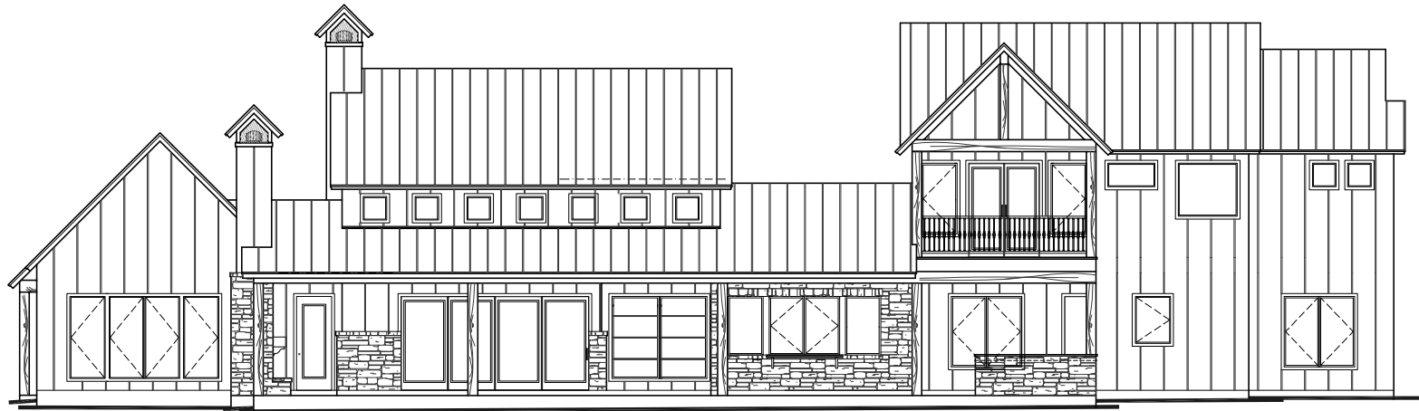
Rear Elevation
