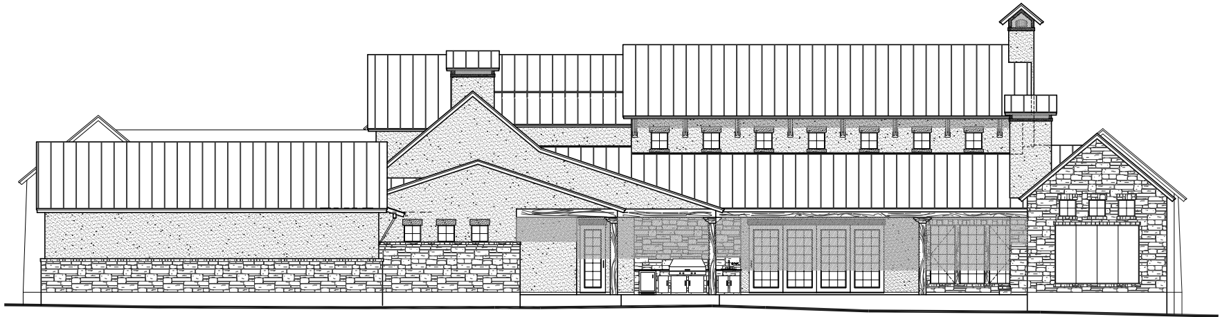
Rear Elevation
